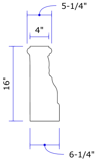
FTN10-ED Side Profile Scale: 1"=1'
