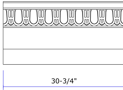
FTN10-ED Front View: Egg and Dart Scale=1"=1'
